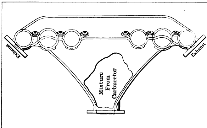
Fig. 15—Manifold of a box-like character, with provision to utilize exhaust heat.
